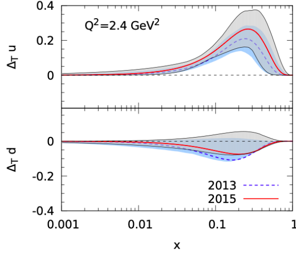
FIG. 7. The extracted u and d transversity distributions in a comparison of the best fit results (red, solid lines). [88].
