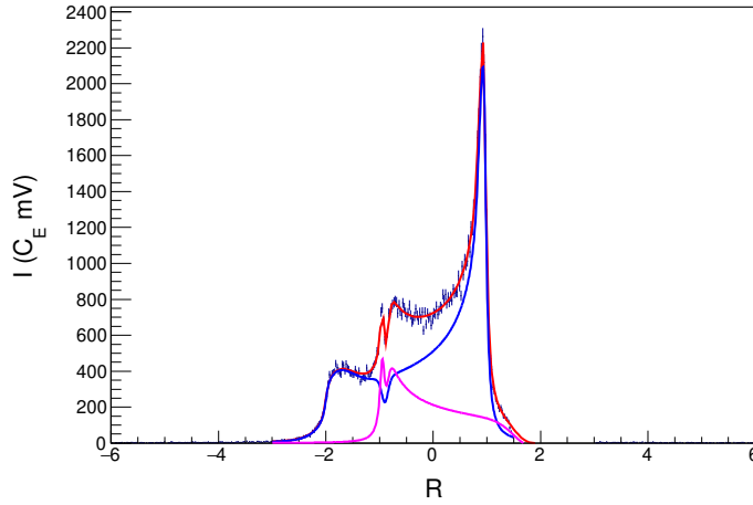
FIG. 21. NMR measurement with fit result after the ss-RF has been applied to the two negative tensor regions. The tensor polarization from this example is about 32%. Figure from [124].
