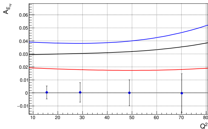
FIG. 26. Projections of the gluon transversity asymmetry with expected data point. Error bars on projected data points are from statistical and systematic uncertainty estimates.
