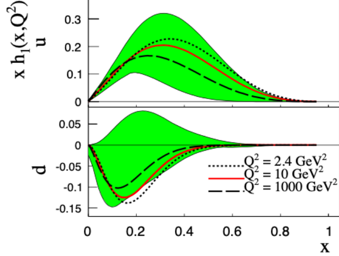
FIG. 6. The extracted transversity distribution at three different scales in Q^2 . The shaded region corresponds to the 90% confidence level error band at Q^2 = 10 \text{ GeV}^2 [84].
