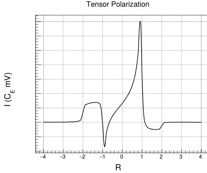
FIG. 20. The tensor polarization shown from the difference of the intensities I_+(R) and I_-(R) . Figure from [124].
